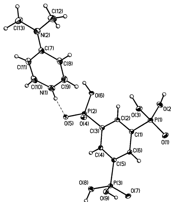
Figure 4. Molecular structure of [\text{1,3-}\{(\text{HO})_2(\text{O})\text{P}\}_2\text{-5-}\{(\text{HO})(\text{O})_2\text{P}\}-\text{C}_6\text{H}_3}]^- [\text{4-(Me}_2\text{N)C}_5\text{H}_4\text{NH}]^+ ( 3 ): view of the building unit of 3 showing the labeling scheme and the thermal ellipsoids drawn at 30% of probability level; selected bond lengths: \text{P(1)}-\text{O(1)} 1.481(1) Å, \text{P(1)}-\text{O(2)} 1.552(2) Å, \text{P(1)}-\text{O(3)} 1.551(1) Å, \text{P(2)}-\text{O(4)} 1.514(1) Å, \text{P(2)}-\text{O(5)} 1.512(1) Å, \text{P(2)}-\text{O(6)} 1.553(1) Å, \text{P(3)}-\text{O(7)} 1.495(1) Å, \text{P(3)}-\text{O(8)} 1.542(1) Å, \text{P(3)}-\text{O(9)} 1.549(1) Å
