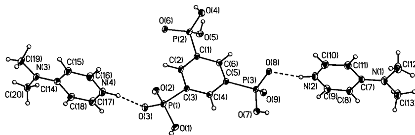
Figure 1. Molecular structure of [1-{(HO) 2 (O)P}-3,5-{(HO)(O) 2 P} 2 -C 6 H 3 ] 2− [{4-(Me 2 N)C 5 H 4 NH} + ] 2 ( 2 ): view of the building unit of 2 showing the labeling scheme and the thermal ellipsoids drawn at 30% of probability level; selected bond lengths: P(1)–O(1) 1.570(2) Å, P(1)–O(2) 1.519(2) Å, P(1)–O(3) 1.495(2) Å, P(2)–O(4) 1.552(2) Å, P(2)–O(5) 1.522(2) Å, P(2)–O(6) 1.500(2) Å, P(3)–O(7) 1.538(2) Å, P(3)–O(8) 1.508(2) Å, P(3)–O(9) 1.524(2) Å
