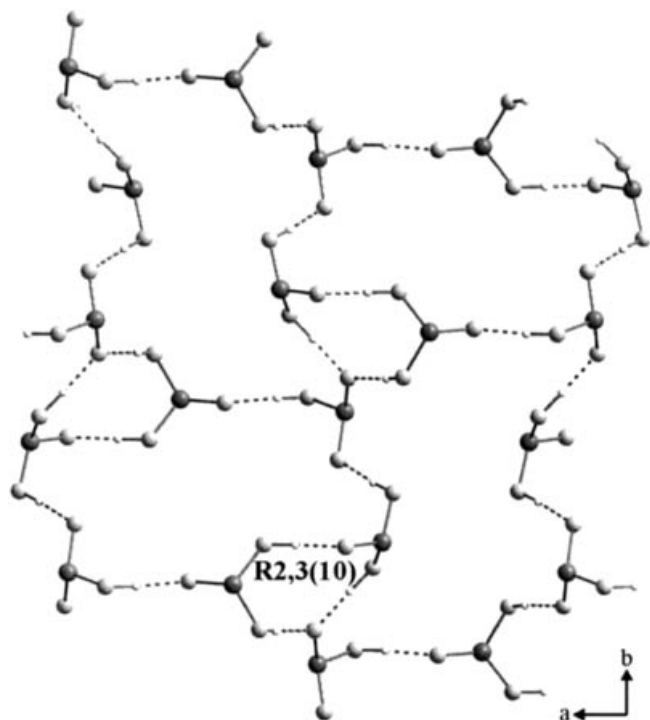
Figure 5. The hydrogen bonded 2-D network of 3 ; view of the a,b plane; the benzene spacer and 4-(dimethylamino)pyridine molecules are omitted for clarity; the main structural motif is a 10-membered ring having the R2,3(10) notation; additional hydrogen bonds link these motifs within the layer; the layers are connected through the benzene spacer along the c axis; (phosphorus: grey; oxygen and hydrogen: light grey)
