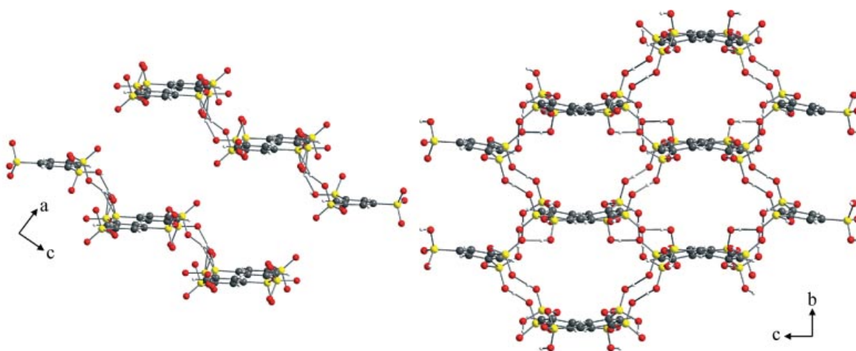
Figure 6. View of the 2-D structure of 2 (left) and the 3-D structure of 3 (right); the cations [4-(\text{Me}_2\text{N})\text{C}_5\text{H}_4\text{NH}]^+ are omitted for clarity (carbon: dark grey; phosphorus: yellow; oxygen: red; hydrogen: light grey)
