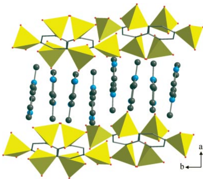
Figure 2. View of the crystal packing diagram of 2 down the c axis showing the layered structure; the cations [\text{4-(Me}_2\text{N)C}_5\text{H}_4\text{NH}]^+ are intercalated between hydrogen-bonded layers (tetrahedron: \text{PO}_3\text{C} ; phosphorus: yellow; carbon: dark grey; nitrogen: blue; oxygen: red)
